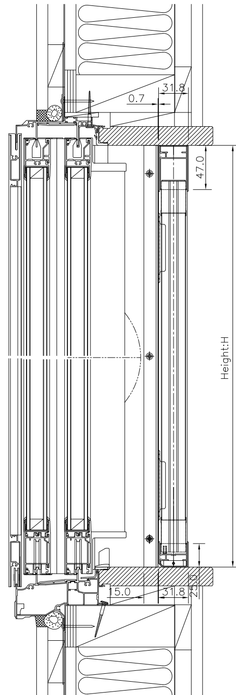
Metaco Pleat Net Front Fix Longitudinal section
