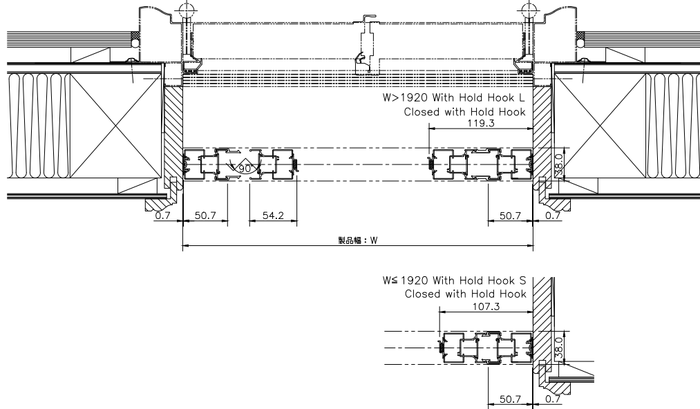
Zipooh Double door (88LME) Cross section
