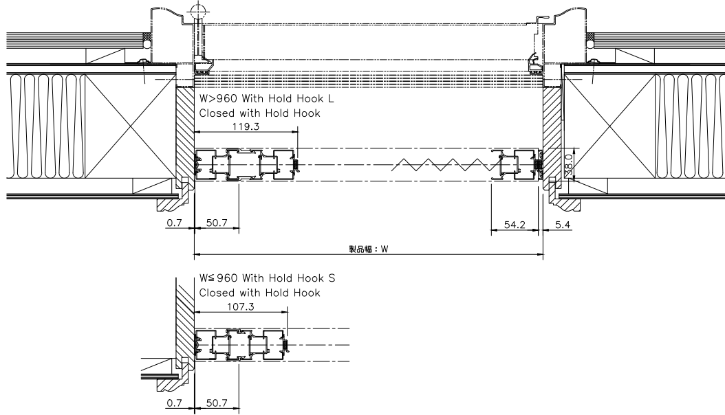
Zipooh Single door (88LME) Cross section
